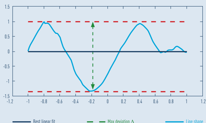
FIG 2 - LINE STRAIGHTNESS
