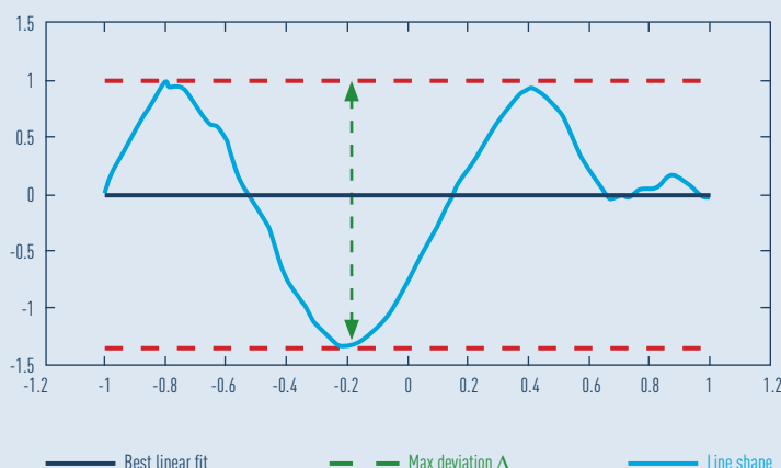
FIG 2 - LINE STRAIGHTNESS
